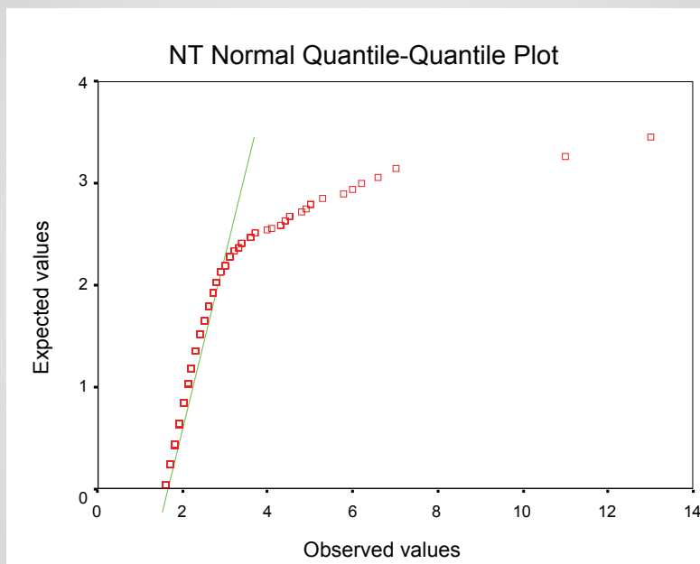
Fig. 1 – Normal quantile-quantile plot of NT values.
